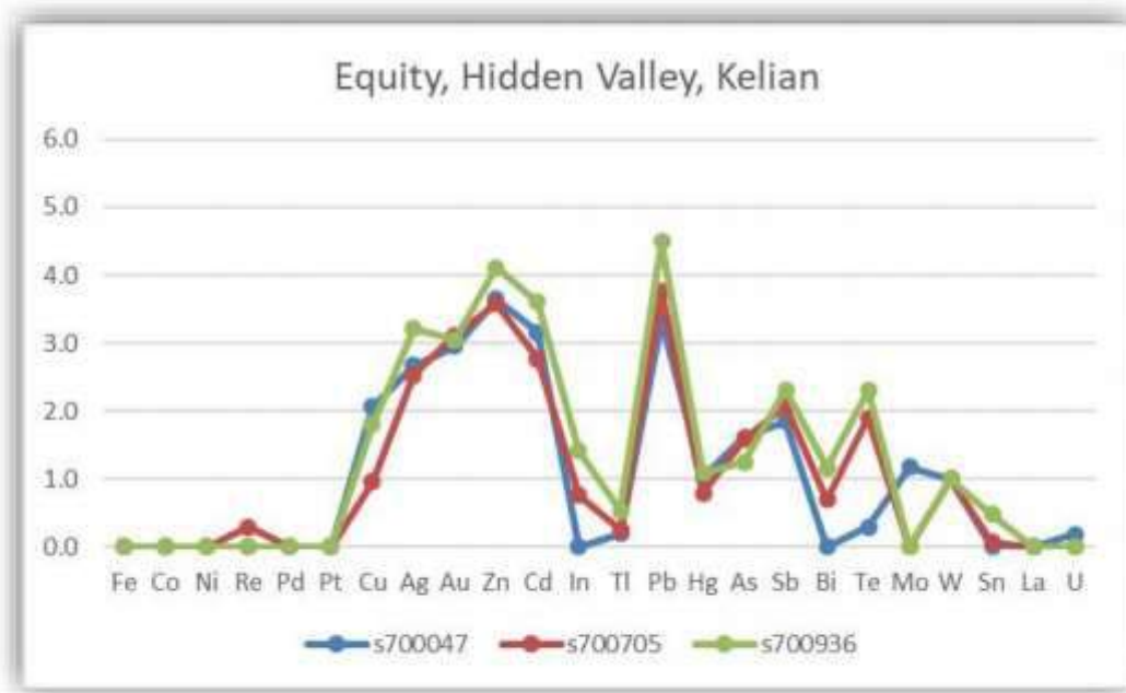
Graph 2: Graph of Geochemistry of Kelian (red), Hidden Valley (green) and Equity (blue) deposits
